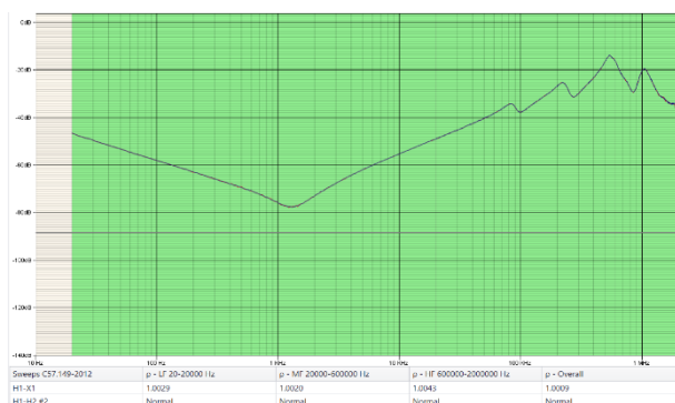
IEEE C57.149-2012 - Graphical comparison of two traces
