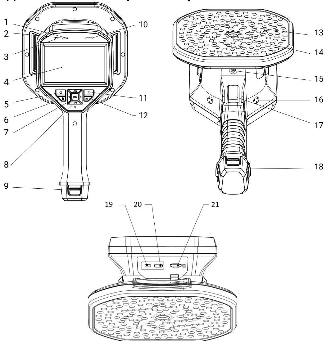
Figure 1-2 Appearance: 136-Microphone Array
