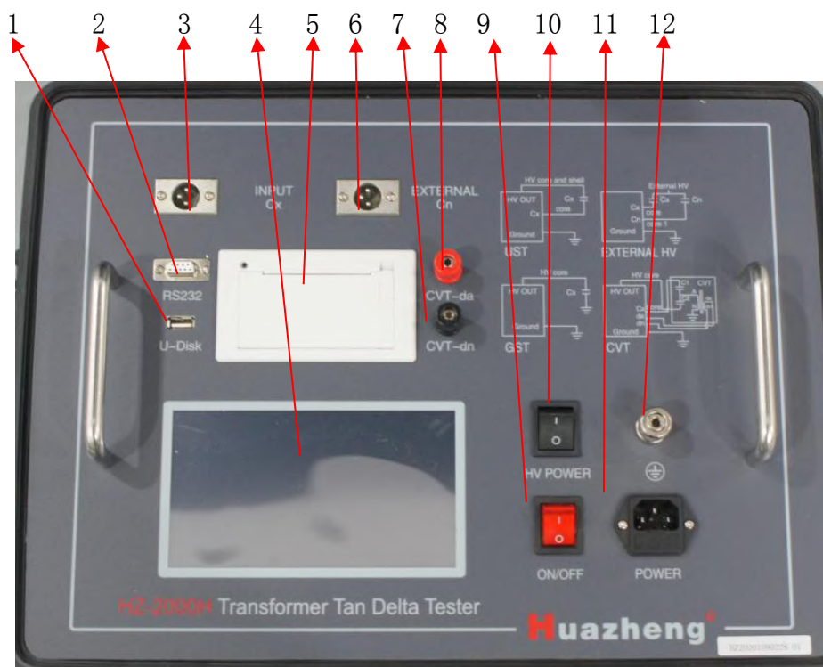
FIG. 9 Instrument panel
