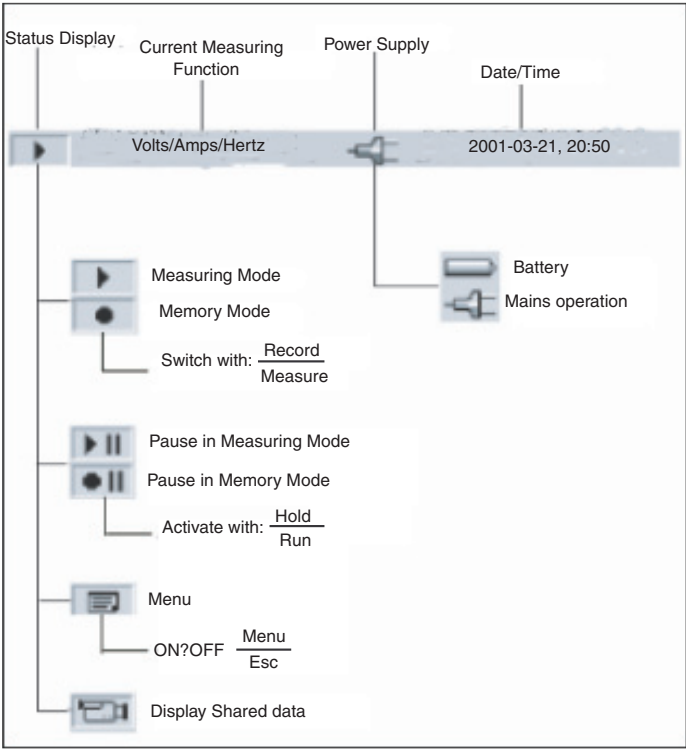
Figure 1. Display Symbols
