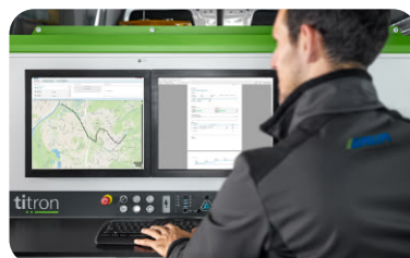
↑ 04 / Software BAUR 4
