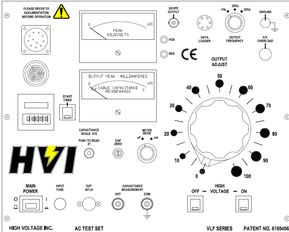
Figure 2 VLF-90 Series front panel controls
